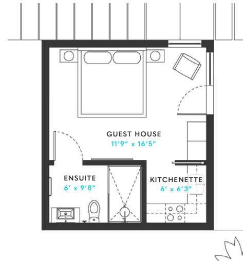
GUEST HOUSE / FOURTH BEDROOM OPTION
